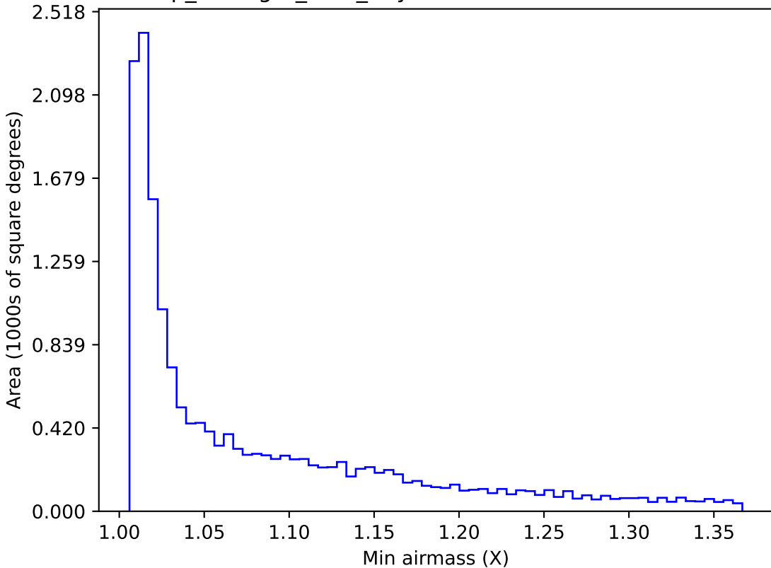
scp_reweight_v3.3_10yrs WFD z band: Min airmass
