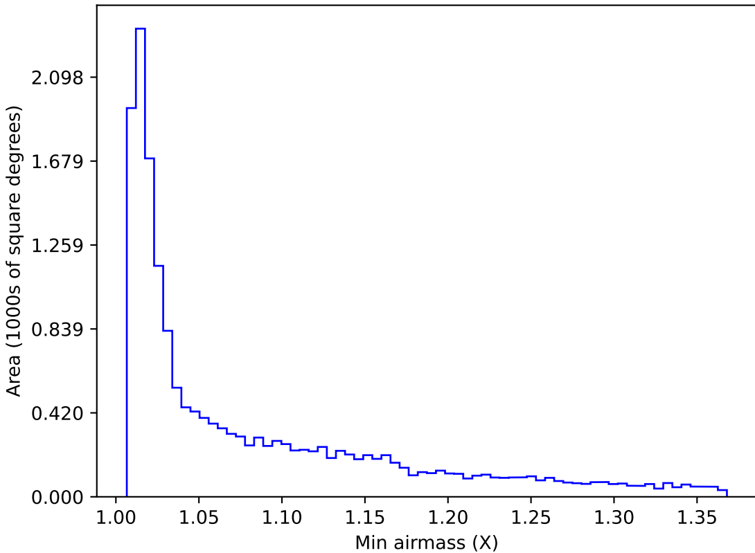
scp_reweight_v3.3_10yrs WFD y band: Min airmass
