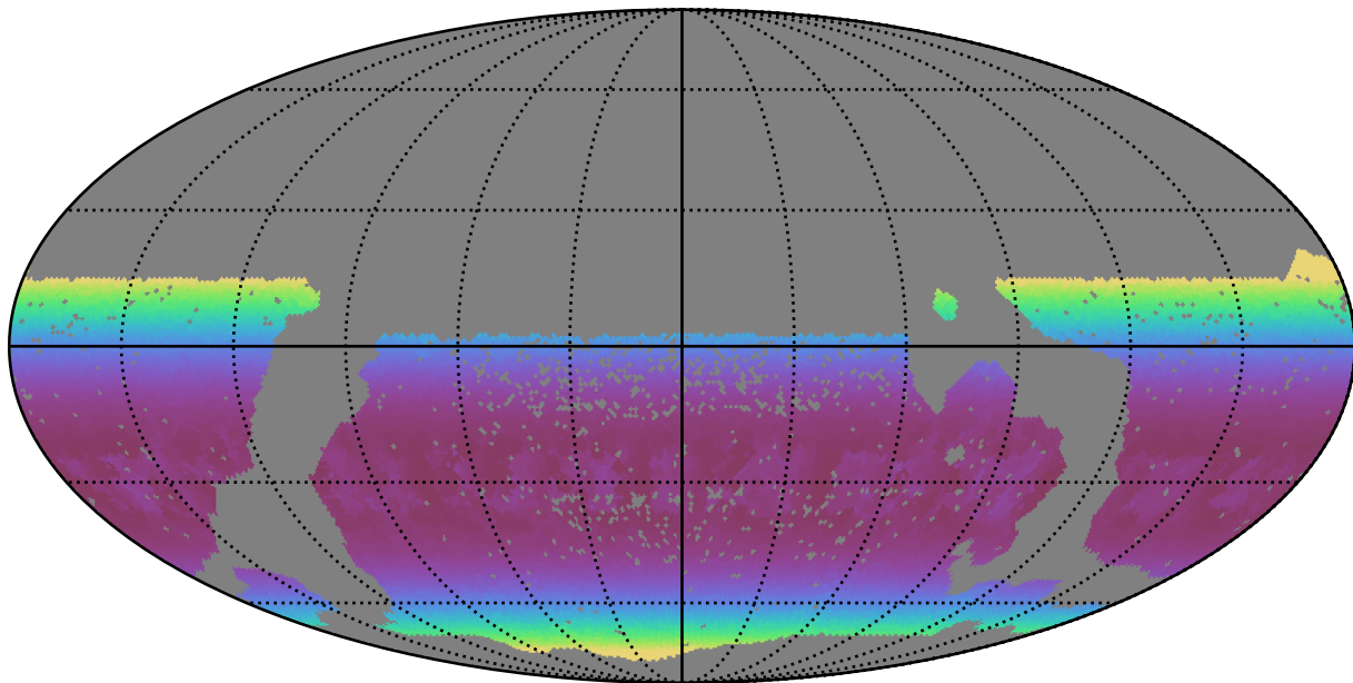
scp_reweight_v3.3_10yrs WFD u band: Min airmass
