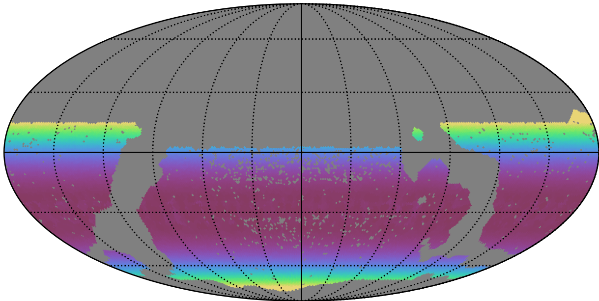
scp_reweight_v3.3_10yrs WFD r band: Min airmass
