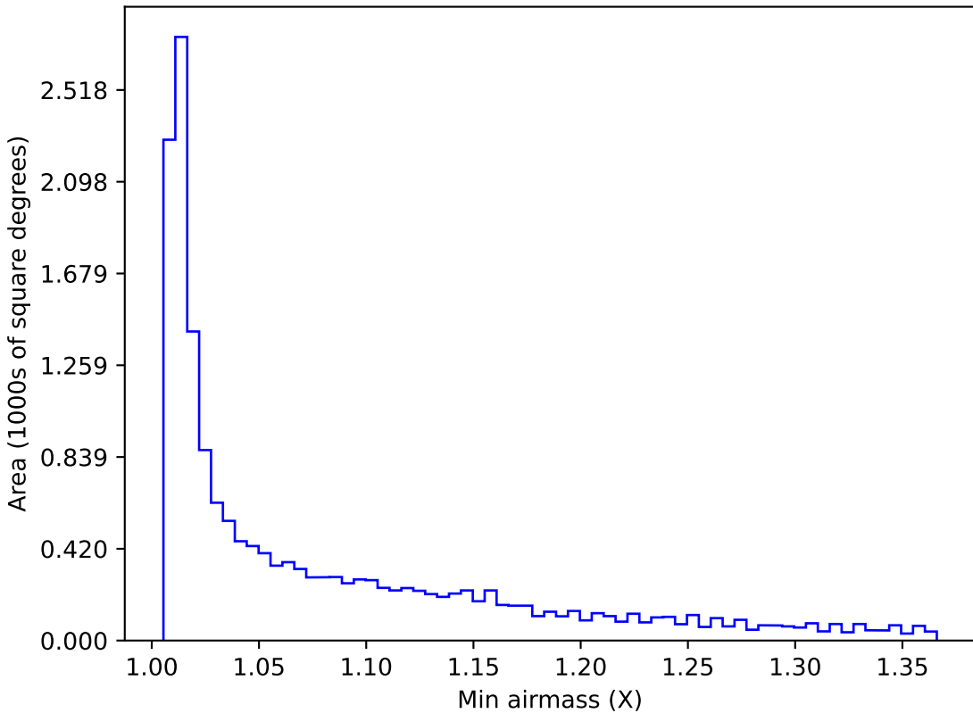
scp_reweight_v3.3_10yrs WFD r band: Min airmass
