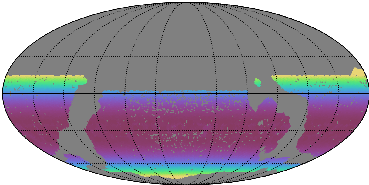
scp_reweight_v3.3_10yrs WFD i band: Min airmass
