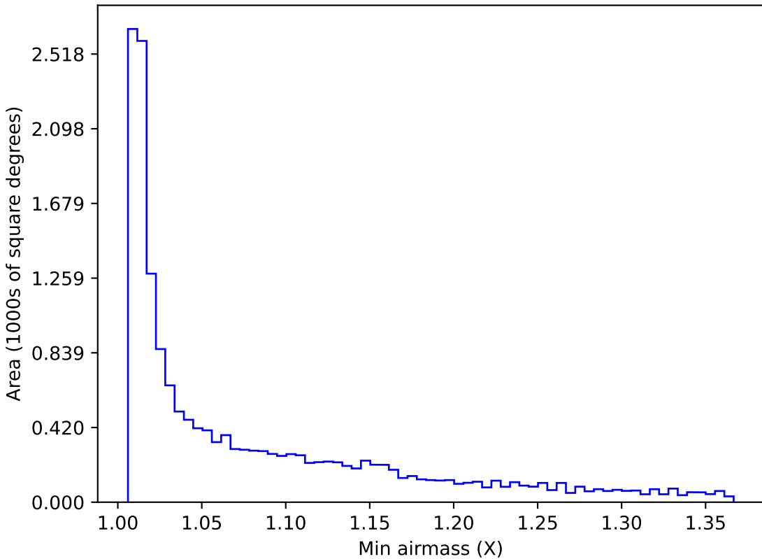
scp_reweight_v3.3_10yrs WFD i band: Min airmass
