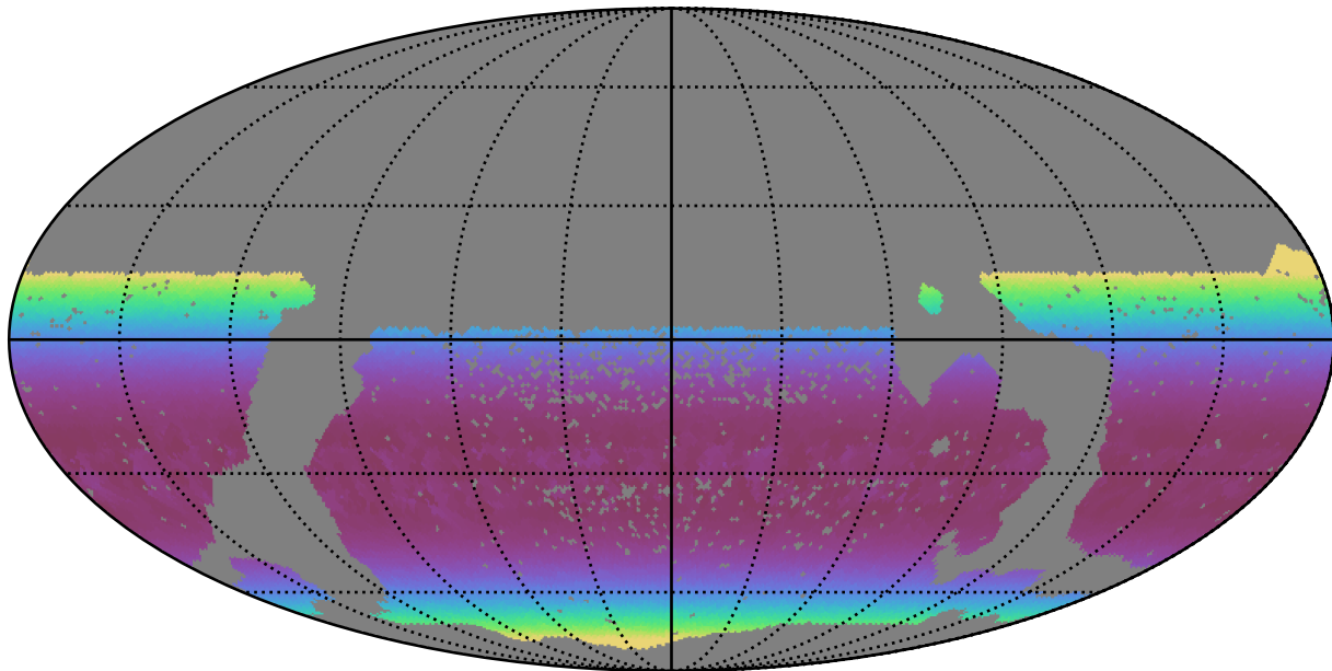
scp_reweight_v3.3_10yrs WFD g band: Min airmass
