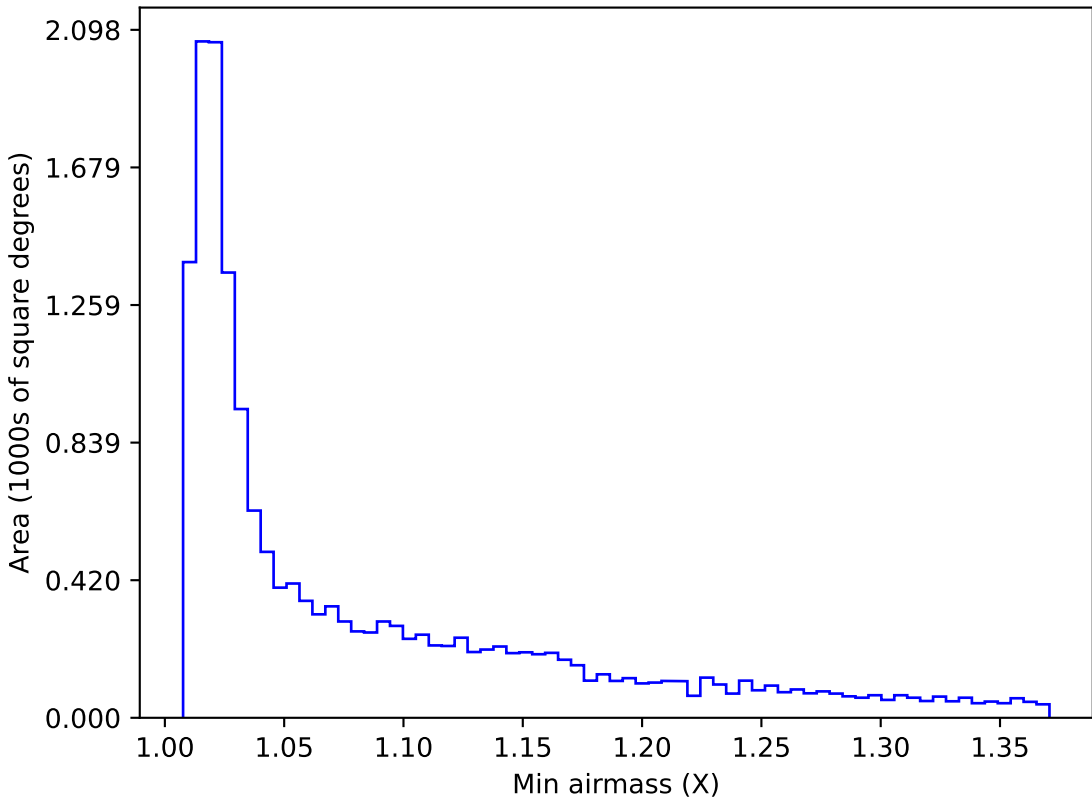
scp_reweight_v3.3_10yrs WFD g band: Min airmass
