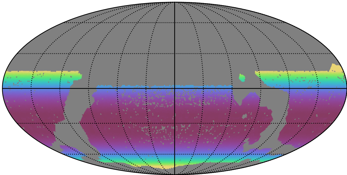
scp_reweight_v3.3_10yrs WFD all bands: Min airmass
