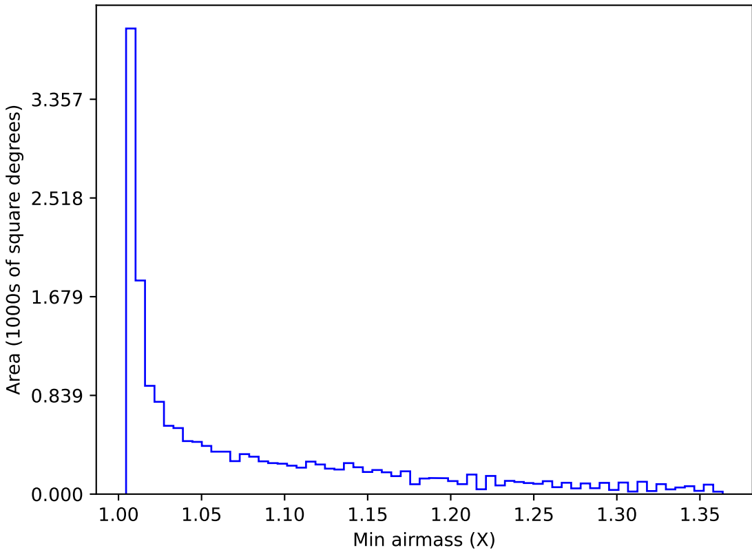
scp_reweight_v3.3_10yrs WFD all bands: Min airmass
