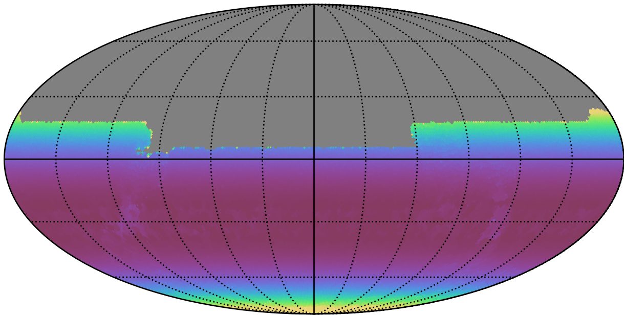
scp_reweight_v3.3_10yrs All sky y band: Min airmass
