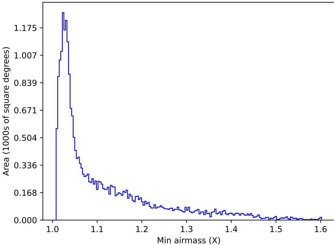
scp_reweight_v3.3_10yrs All sky u band: Min airmass
