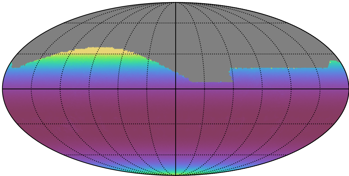
scp_reweight_v3.3_10yrs All sky r band: Min airmass
