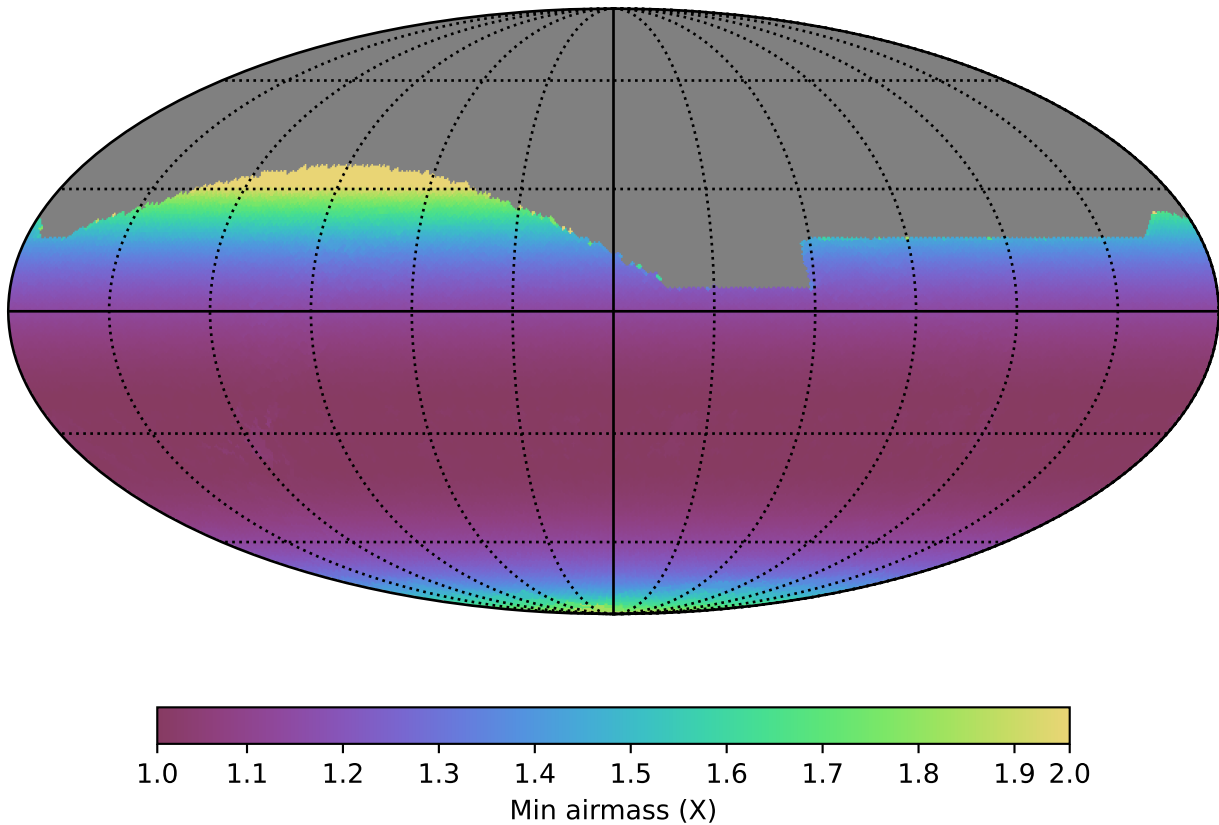
scp_reweight_v3.3_10yrs All sky i band: Min airmass
