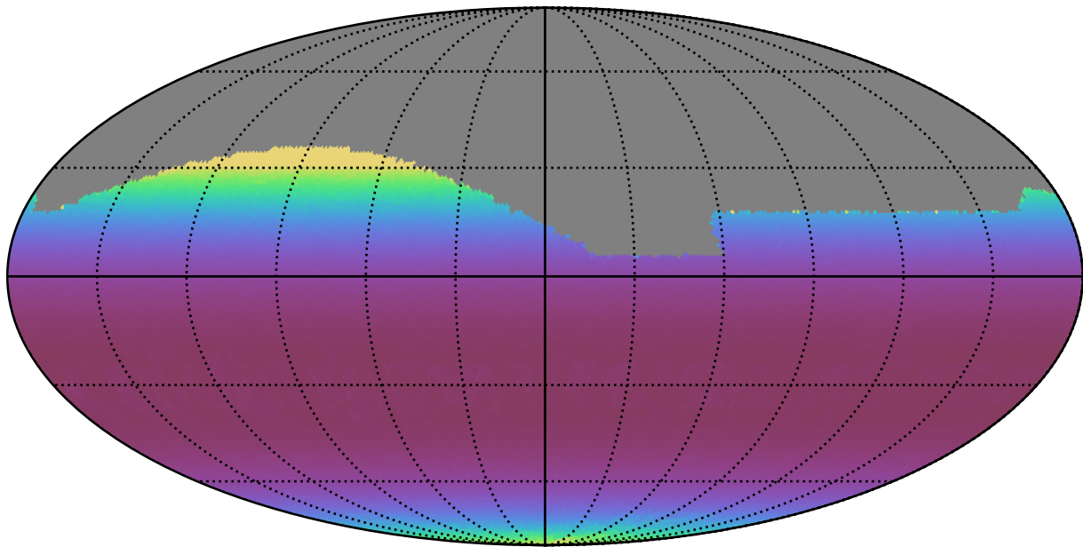
scp_reweight_v3.3_10yrs All sky g band: Min airmass
