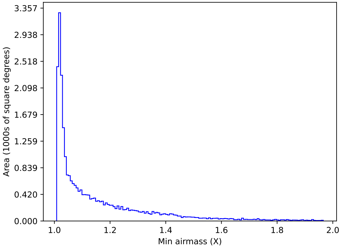
scp_reweight_v3.3_10yrs All sky g band: Min airmass
