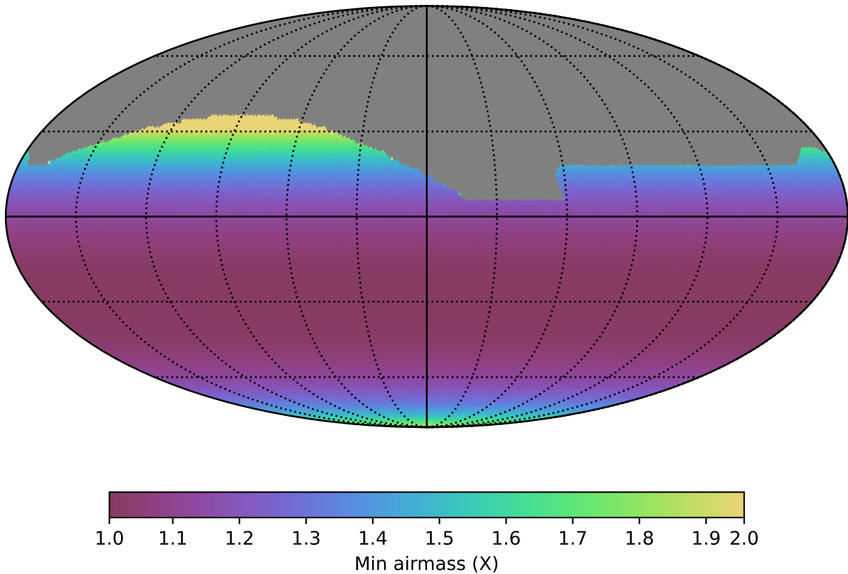
scp_reweight_v3.3_10yrs All sky all bands: Min airmass
