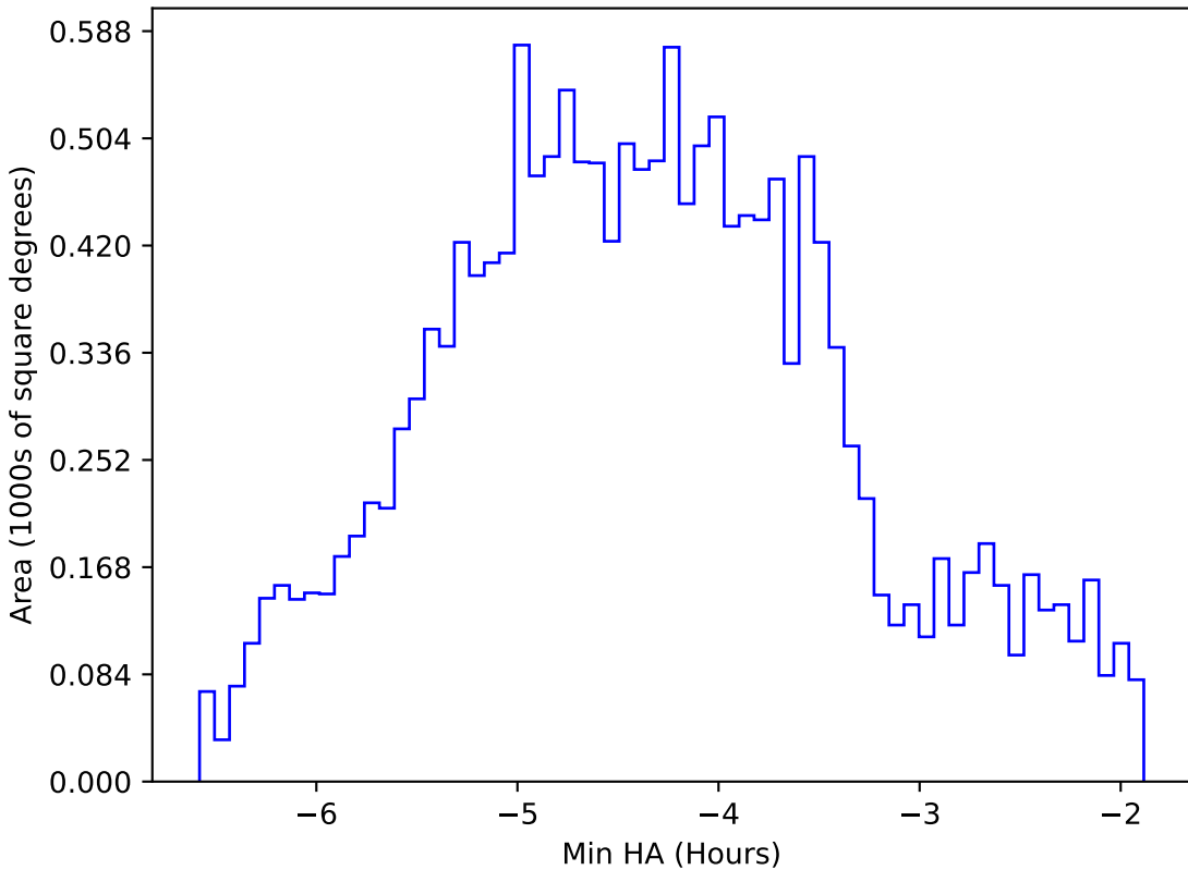
scp_reweight_v3.3_10yrs WFD z band: Min HA
