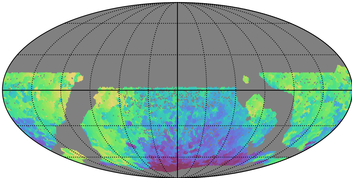
scp_reweight_v3.3_10yrs WFD y band: Min HA
