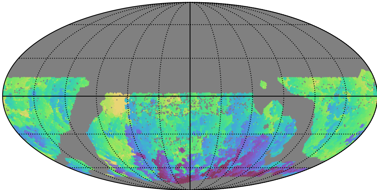
scp_reweight_v3.3_10yrs WFD u band: Min HA
