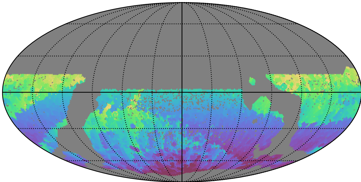
scp_reweight_v3.3_10yrs WFD r band: Min HA
