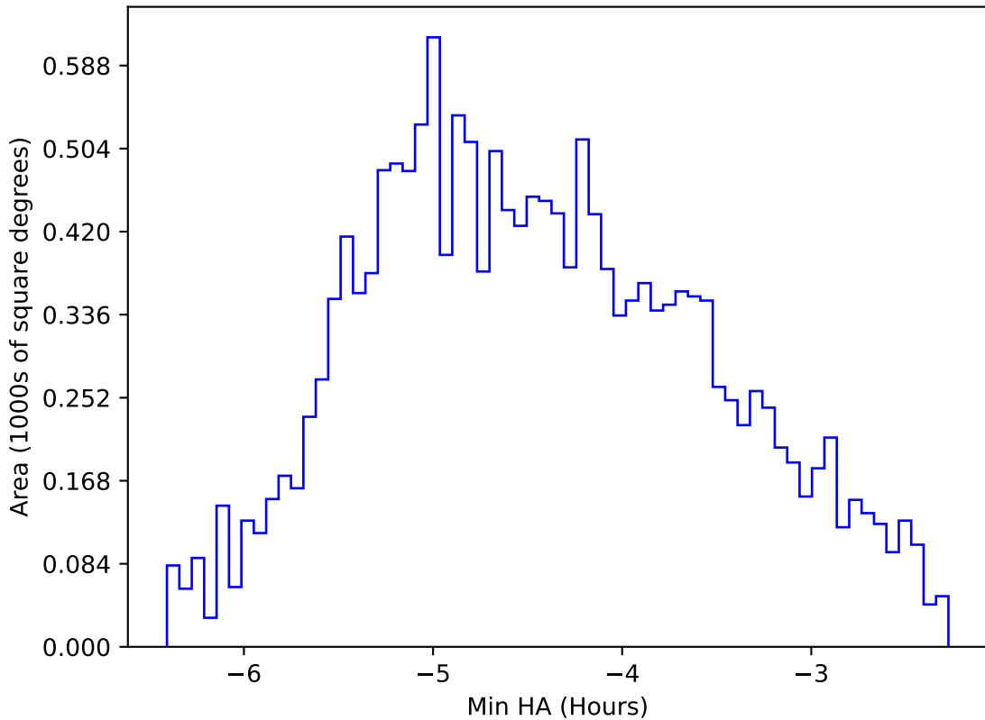
scp_reweight_v3.3_10yrs WFD r band: Min HA
