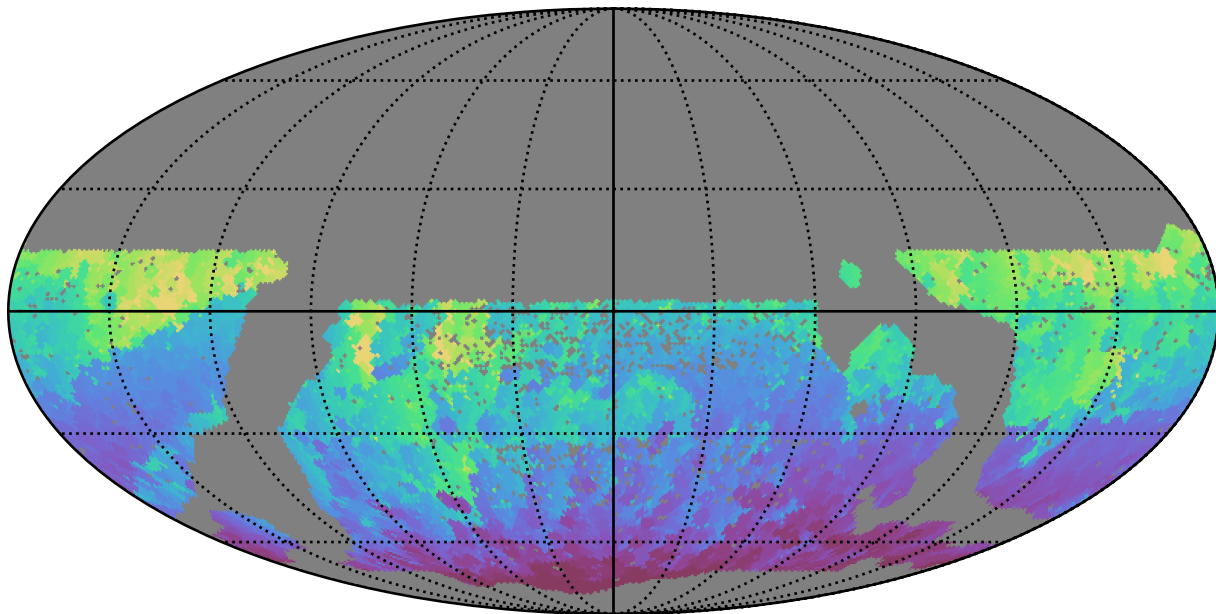
scp_reweight_v3.3_10yrs WFD i band: Min HA
