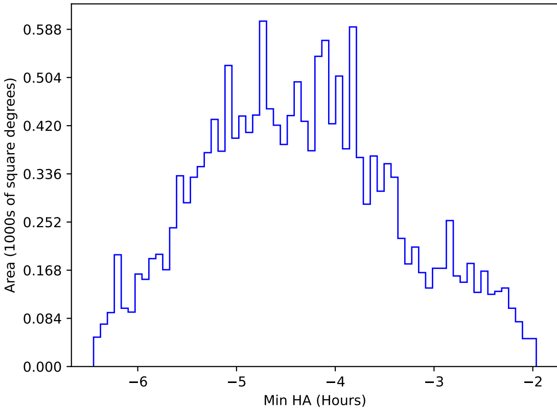
scp_reweight_v3.3_10yrs WFD i band: Min HA
