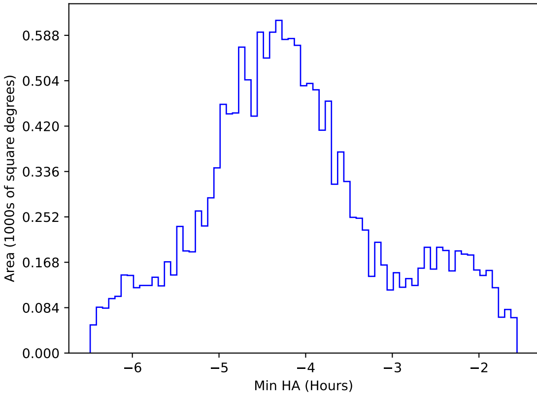
scp_reweight_v3.3_10yrs WFD g band: Min HA
