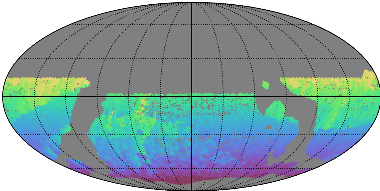
scp_reweight_v3.3_10yrs WFD all bands: Min HA
