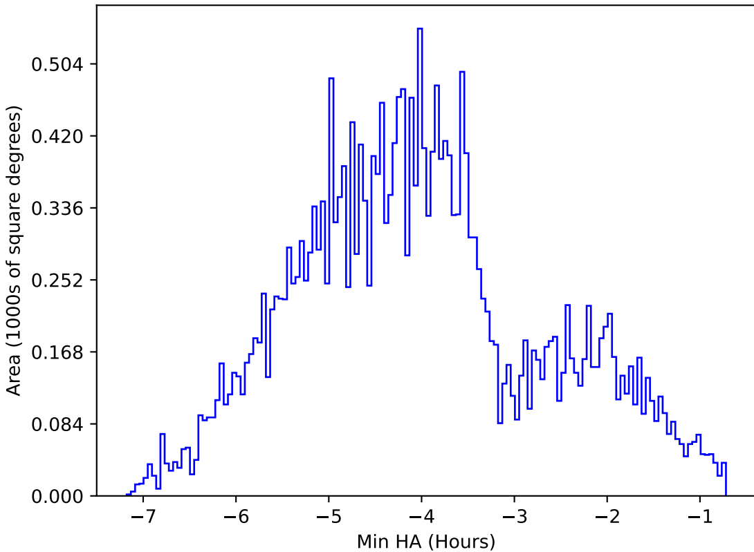
scp_reweight_v3.3_10yrs All sky z band: Min HA
