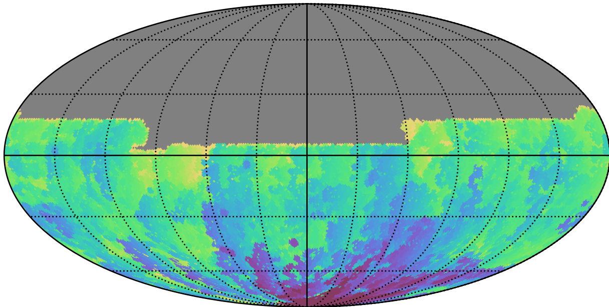
scp_reweight_v3.3_10yrs All sky u band: Min HA
