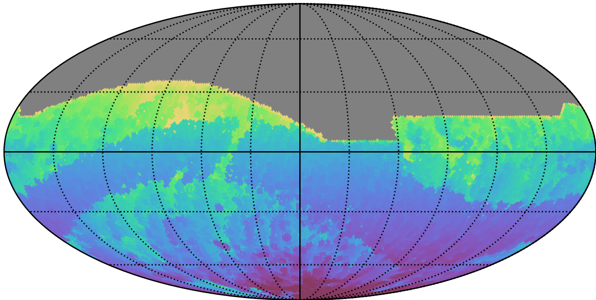
scp_reweight_v3.3_10yrs All sky r band: Min HA
