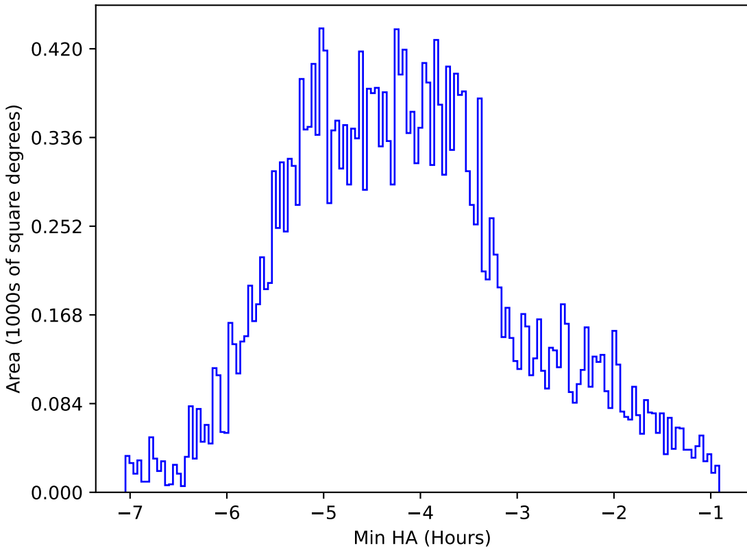
scp_reweight_v3.3_10yrs All sky r band: Min HA
