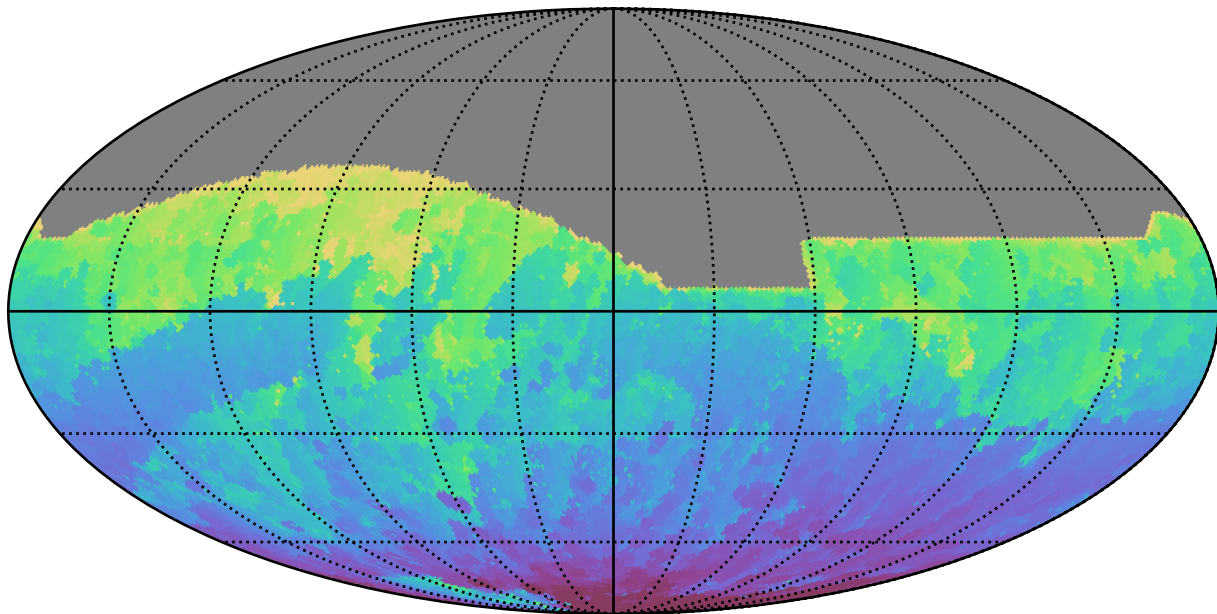
scp_reweight_v3.3_10yrs All sky i band: Min HA
