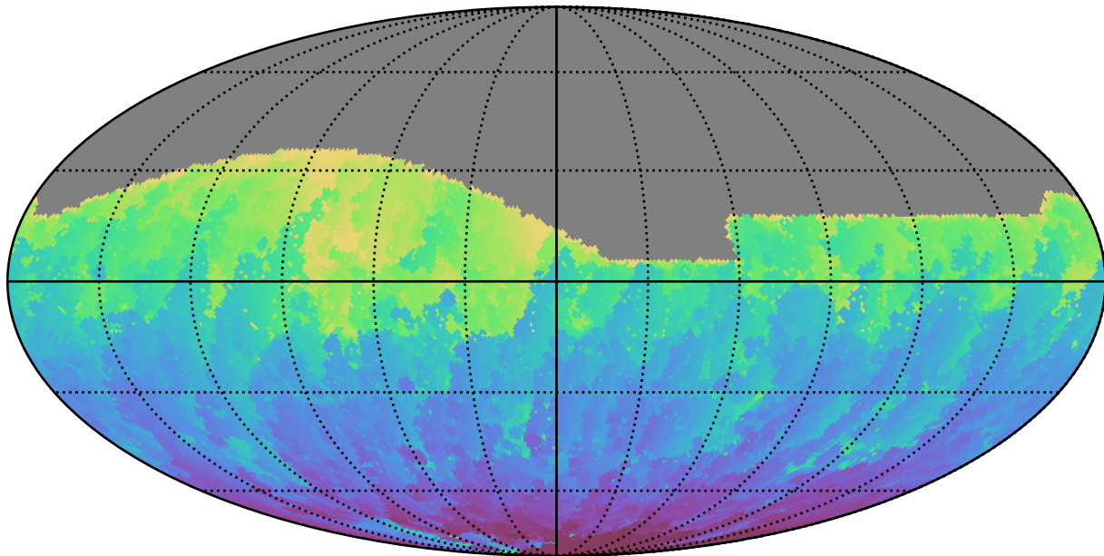
scp_reweight_v3.3_10yrs All sky g band: Min HA
