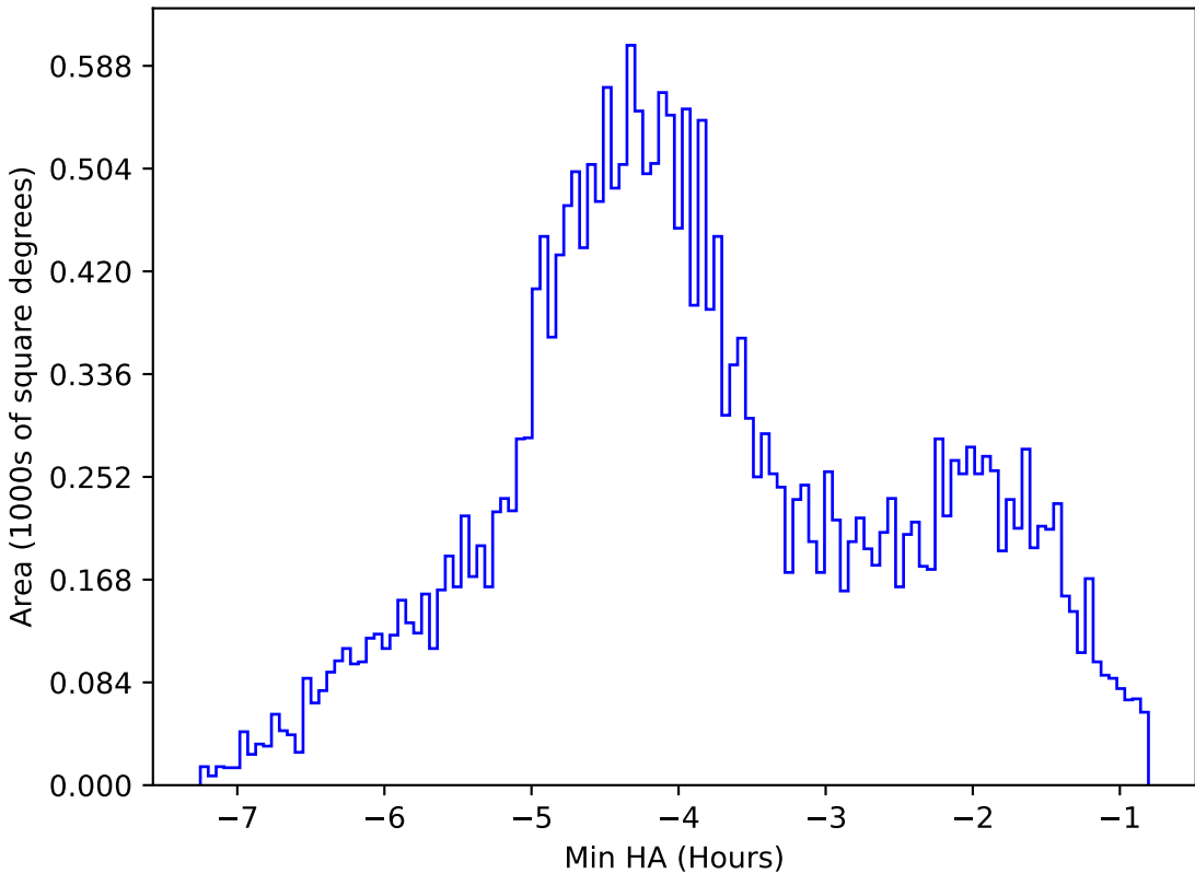
scp_reweight_v3.3_10yrs All sky g band: Min HA
