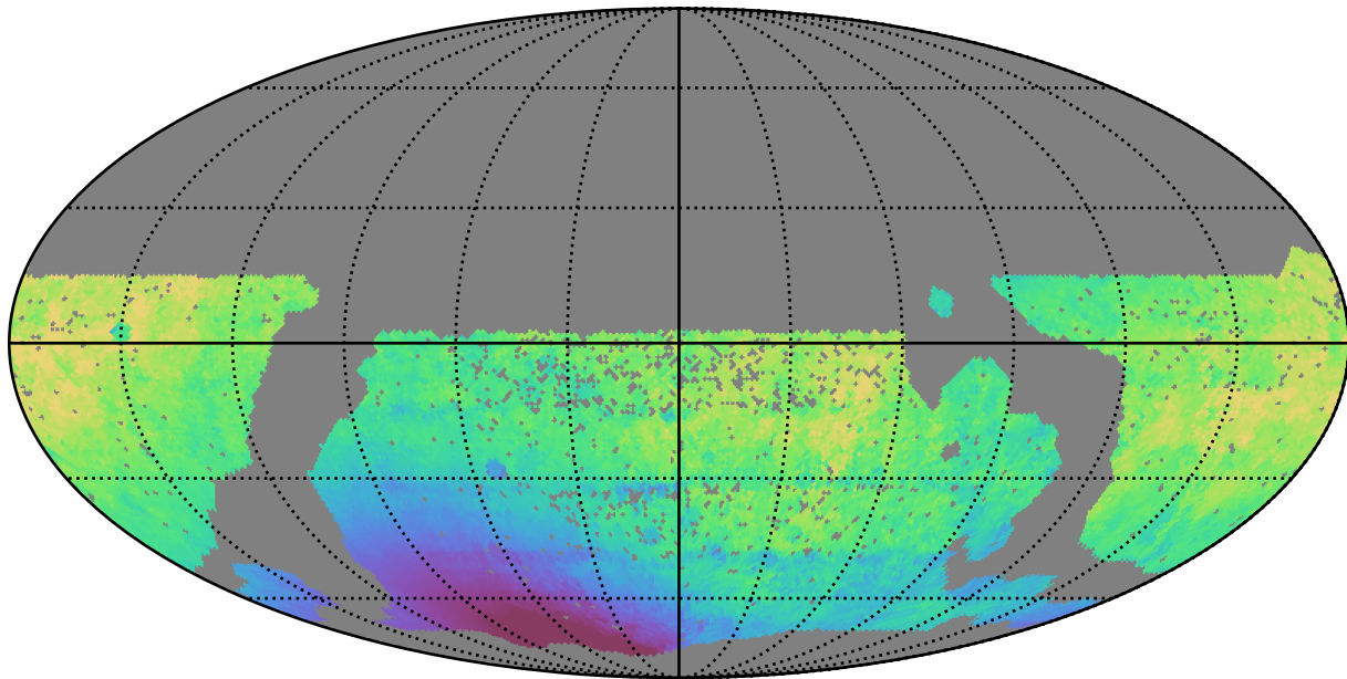
scp_reweight_v3.3_10yrs WFD z band: Median solarElong
