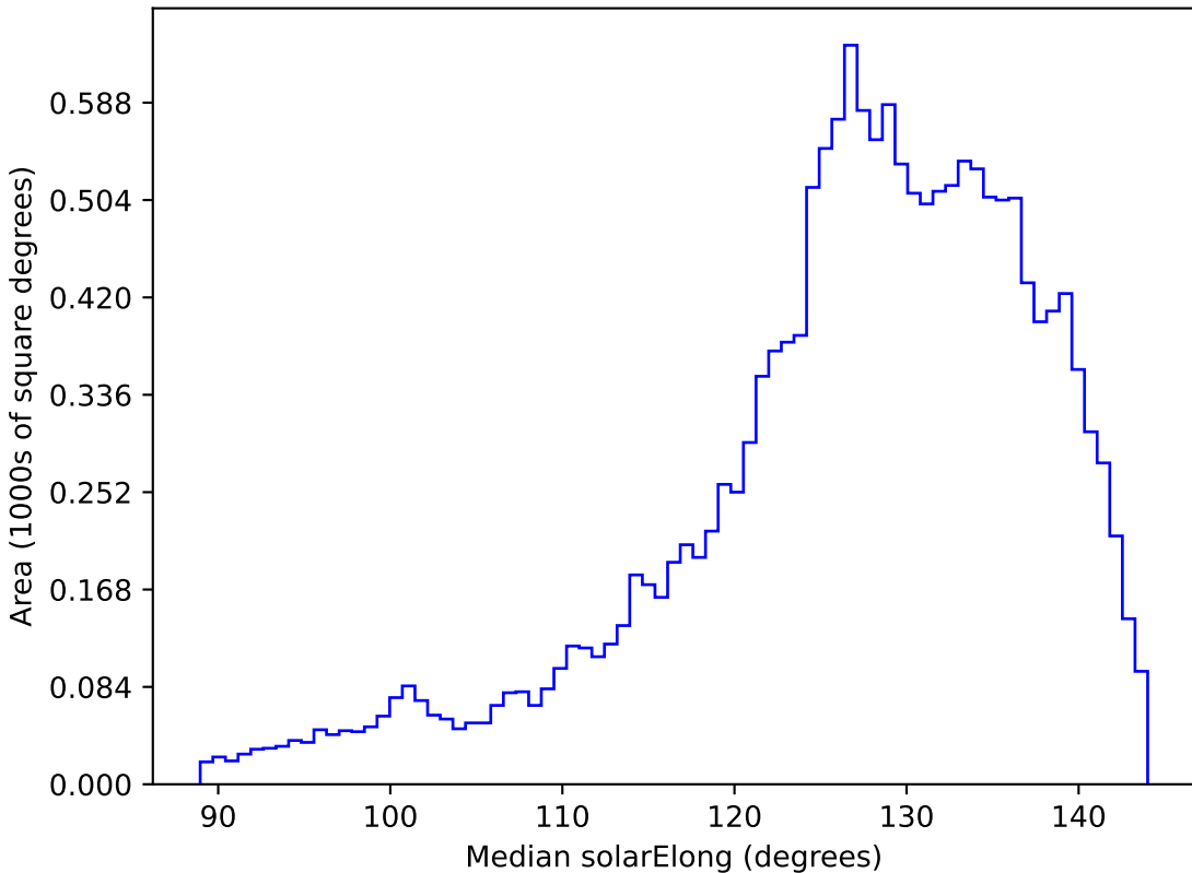
scp_reweight_v3.3_10yrs WFD z band: Median solarElong
