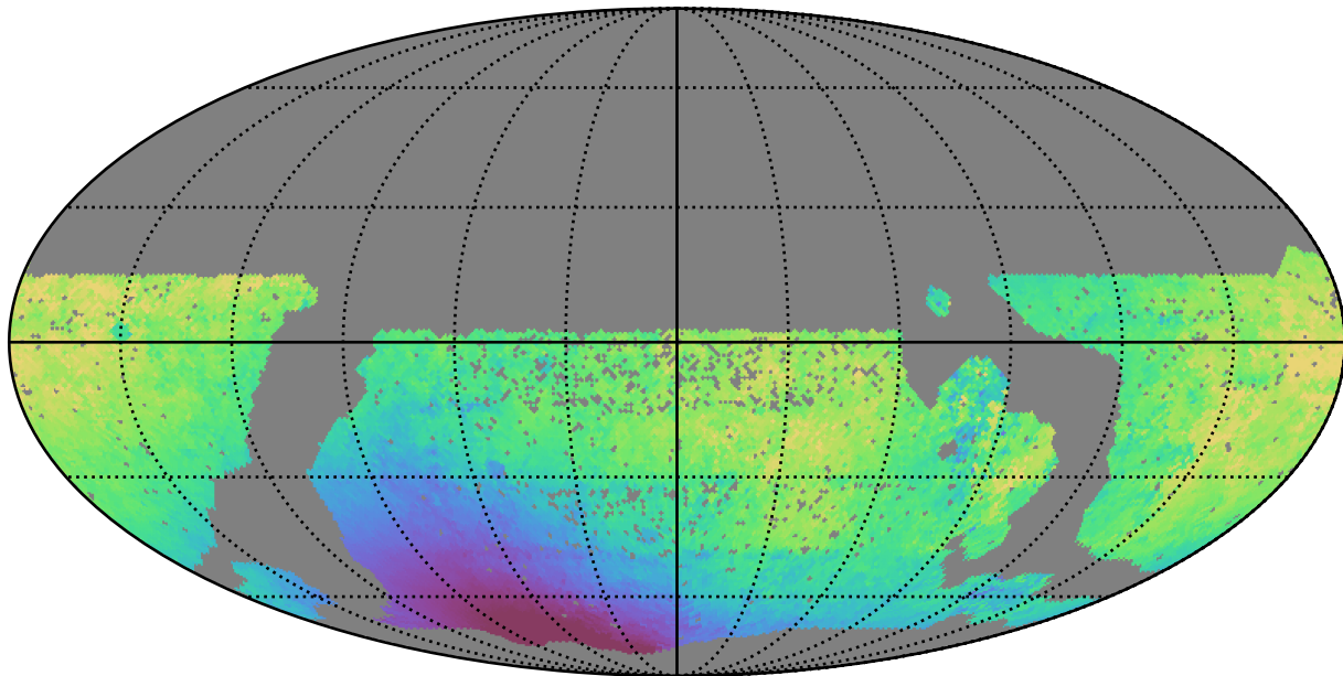
scp_reweight_v3.3_10yrs WFD y band: Median solarElong
