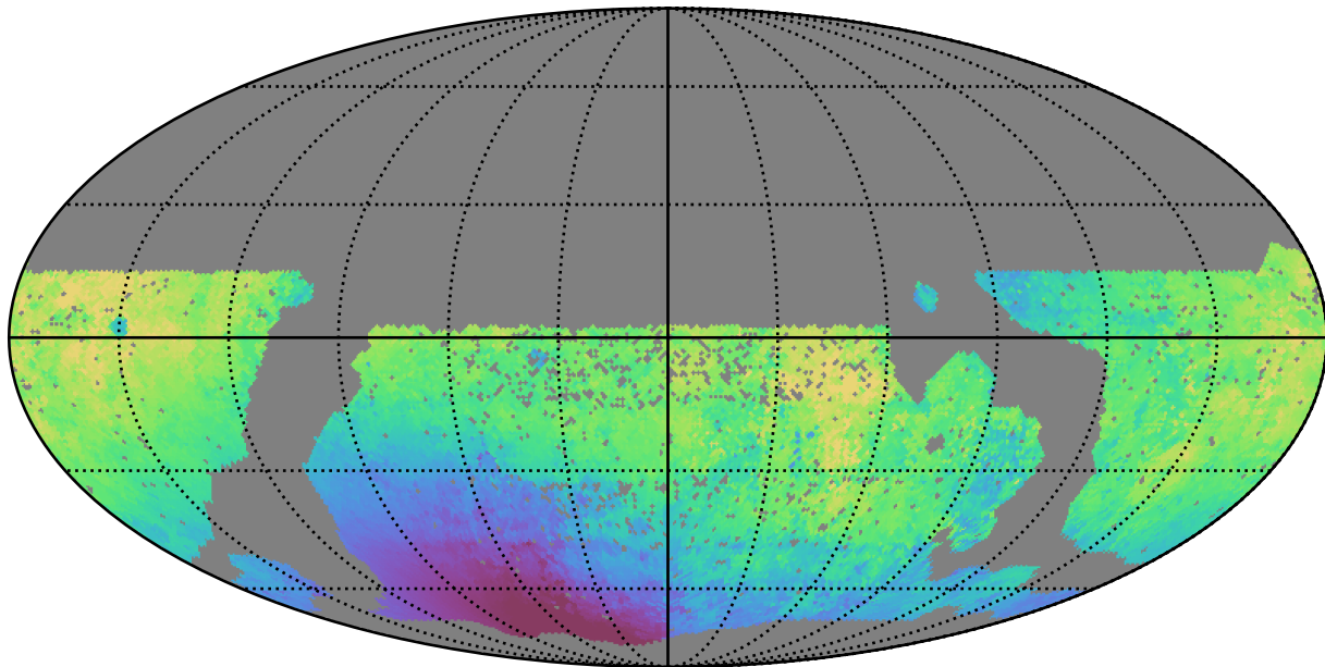
scp_reweight_v3.3_10yrs WFD u band: Median solarElong
