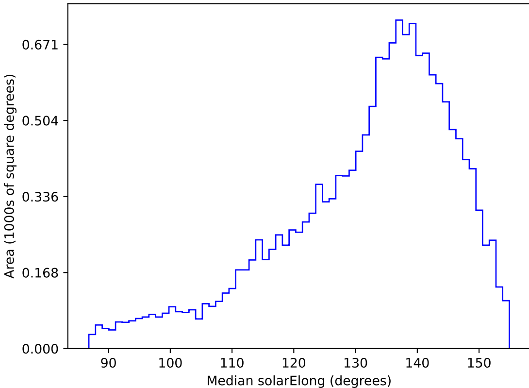
scp_reweight_v3.3_10yrs WFD u band: Median solarElong
