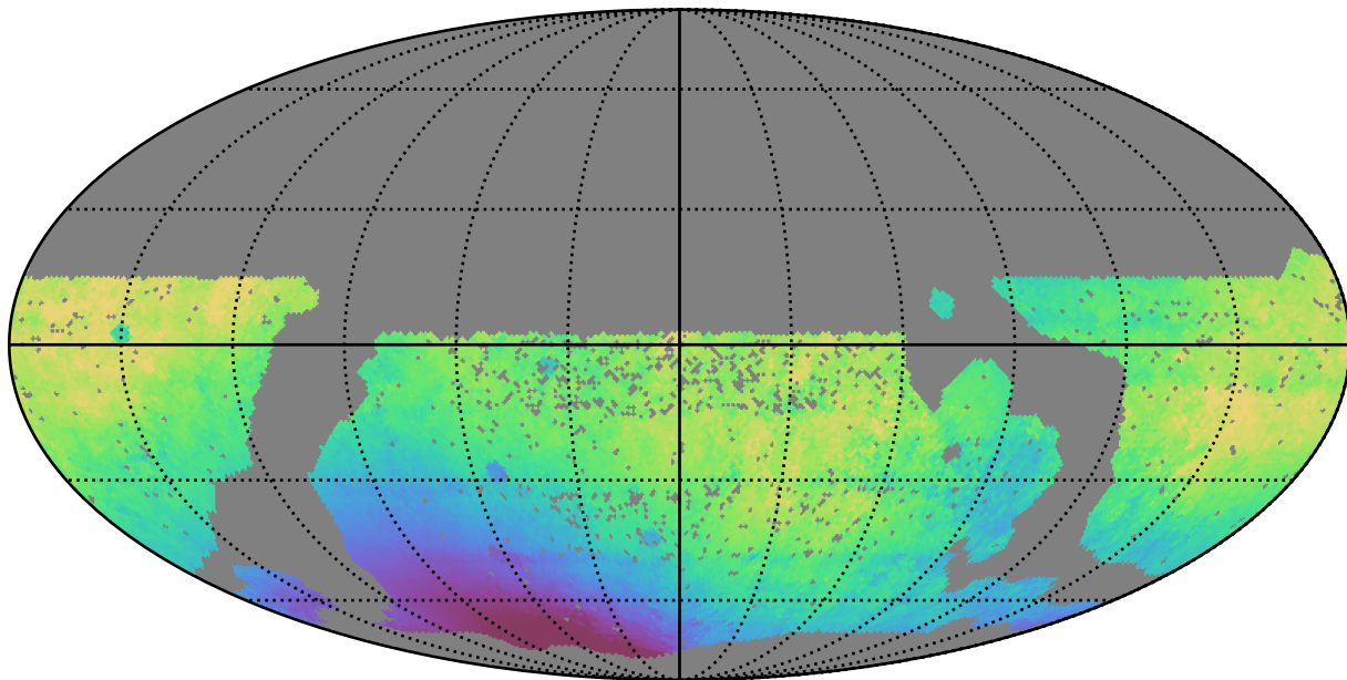
scp_reweight_v3.3_10yrs WFD r band: Median solarElong
