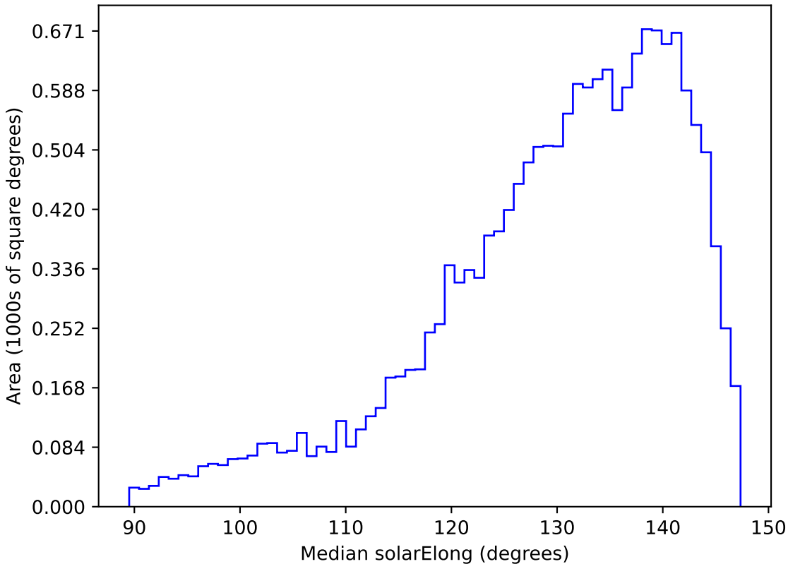
scp_reweight_v3.3_10yrs WFD r band: Median solarElong
