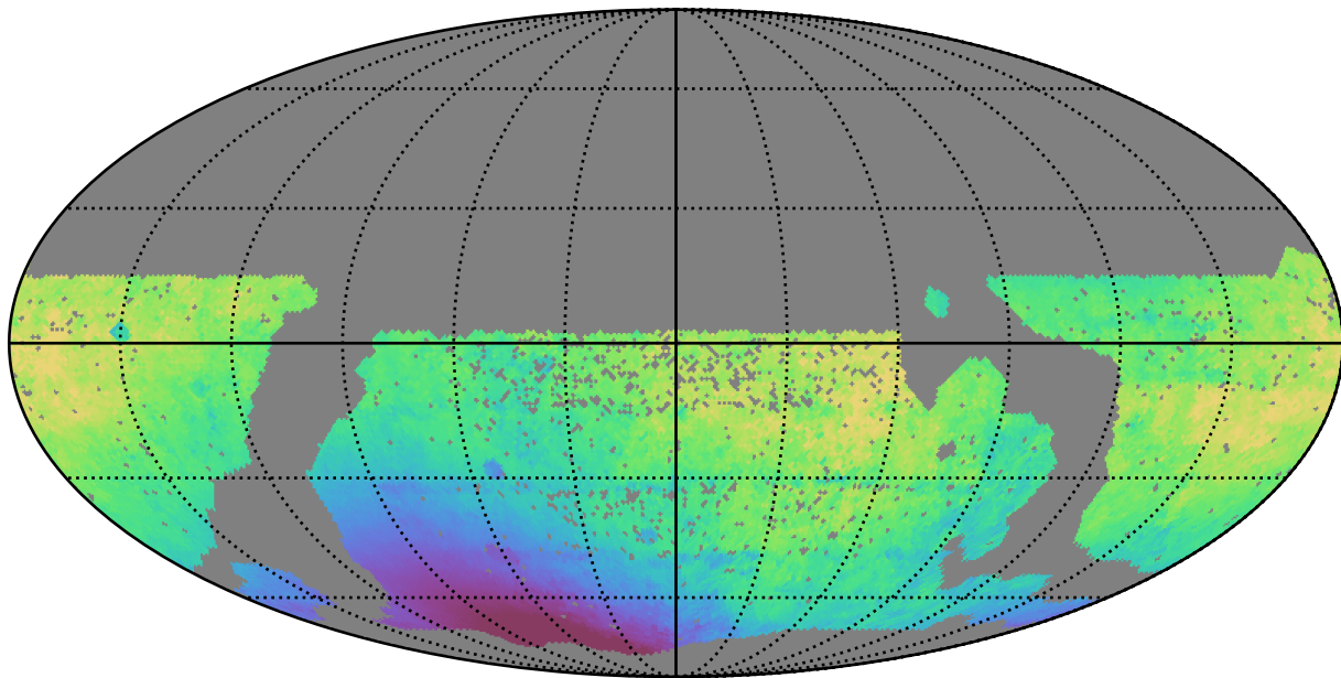
scp_reweight_v3.3_10yrs WFD i band: Median solarElong
