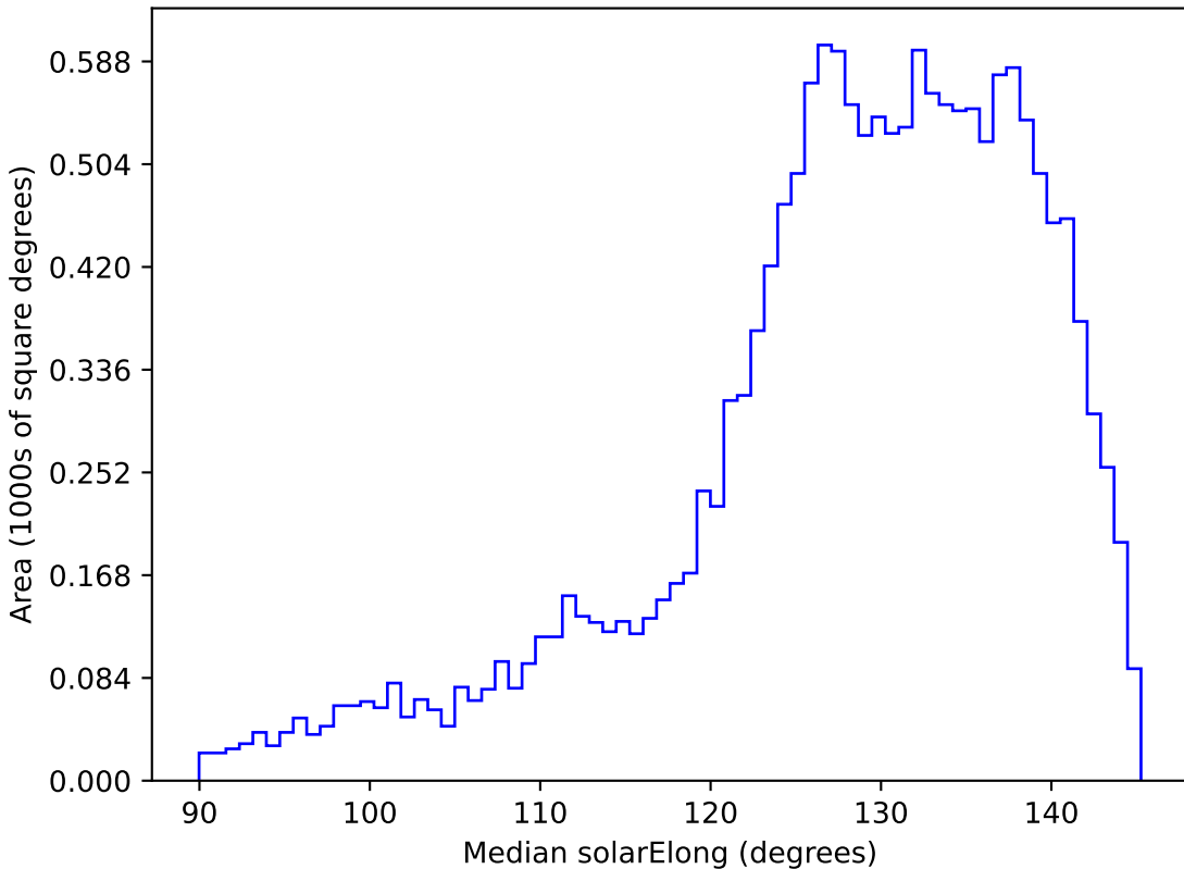
scp_reweight_v3.3_10yrs WFD i band: Median solarElong
