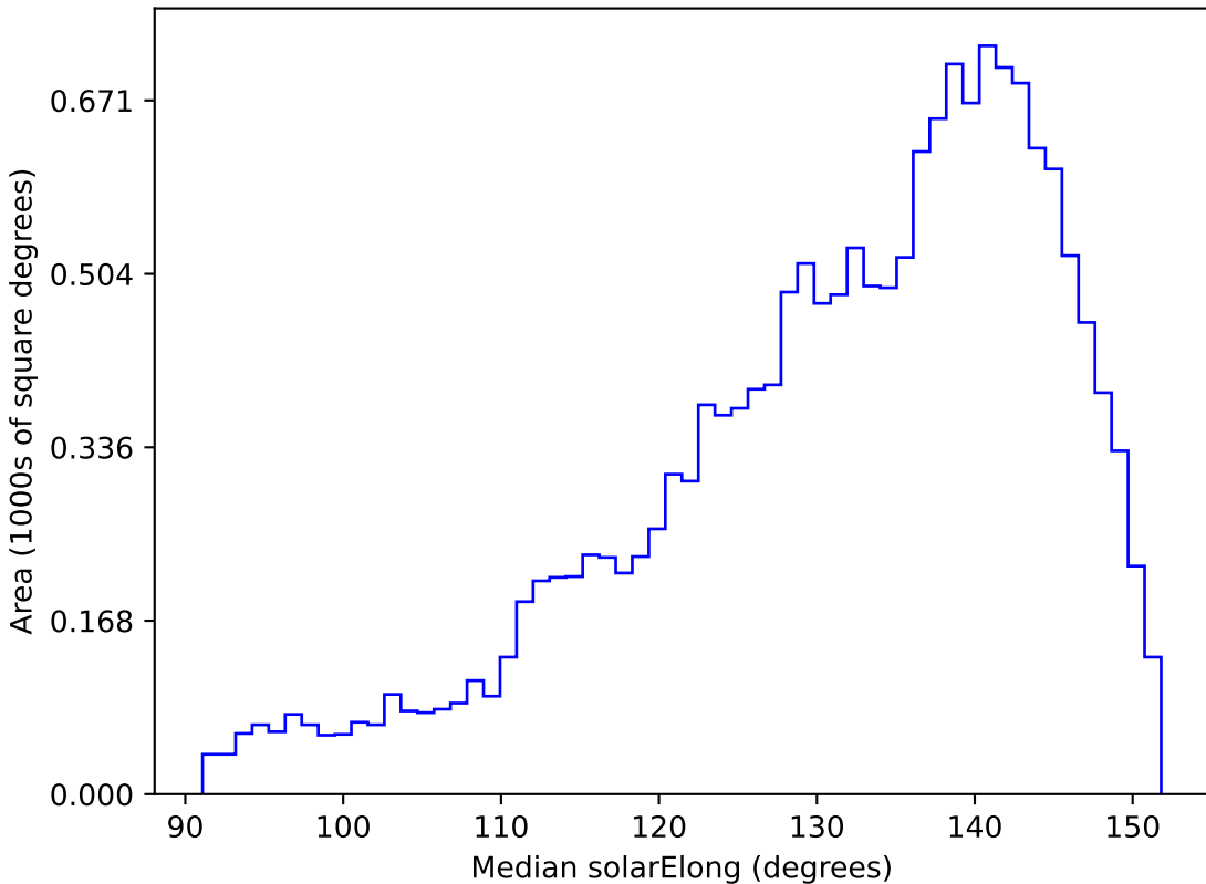
scp_reweight_v3.3_10yrs WFD g band: Median solarElong
