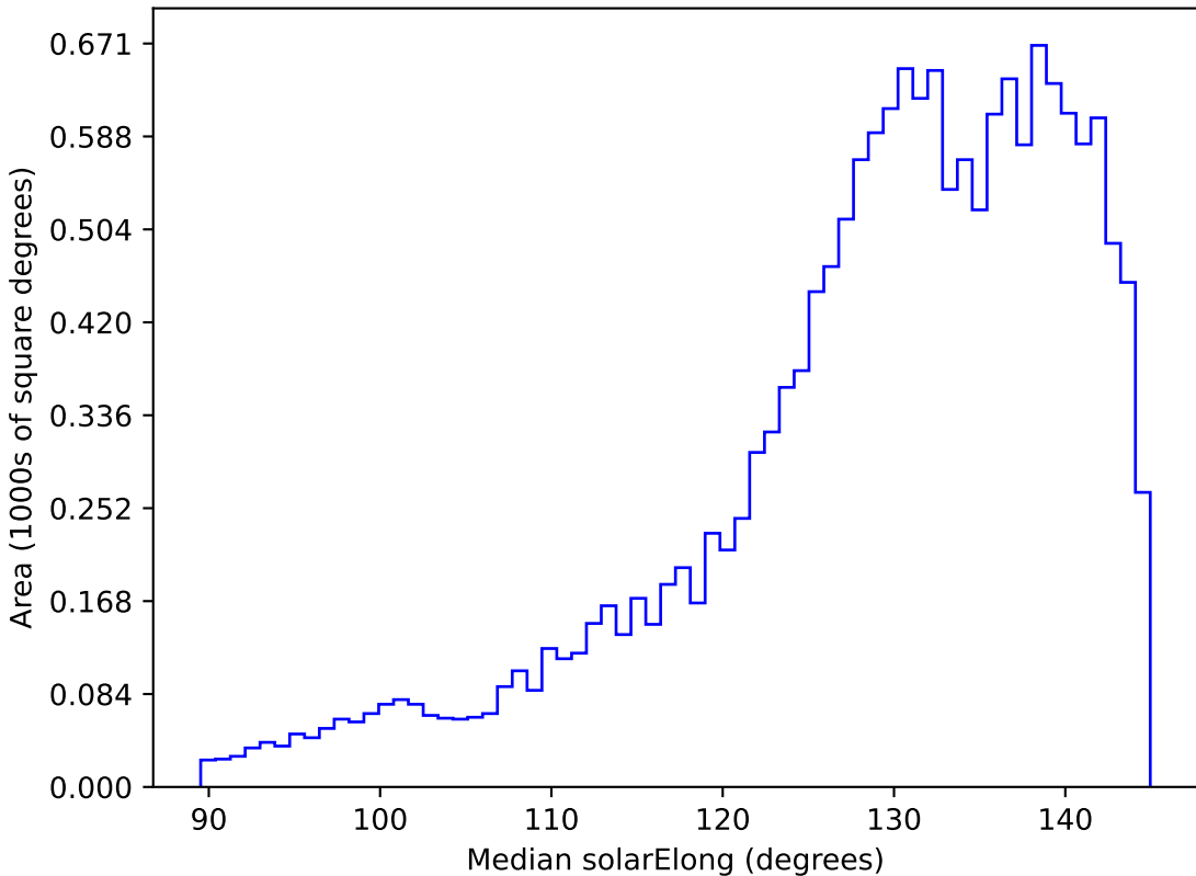
scp_reweight_v3.3_10yrs WFD all bands: Median solarElong
