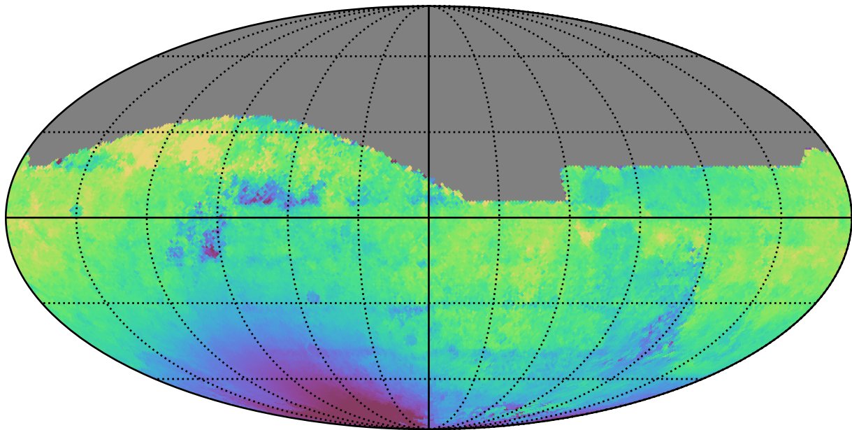
scp_reweight_v3.3_10yrs All sky z band: Median solarElong
