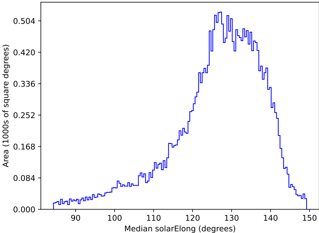
scp_reweight_v3.3_10yrs All sky z band: Median solarElong
