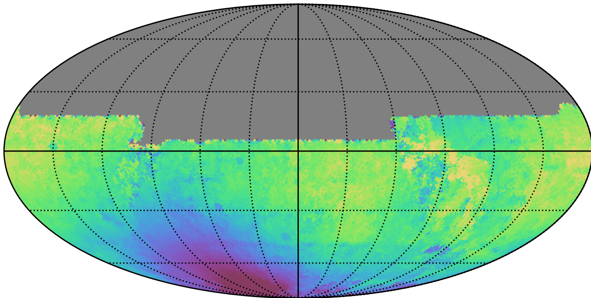
scp_reweight_v3.3_10yrs All sky y band: Median solarElong
