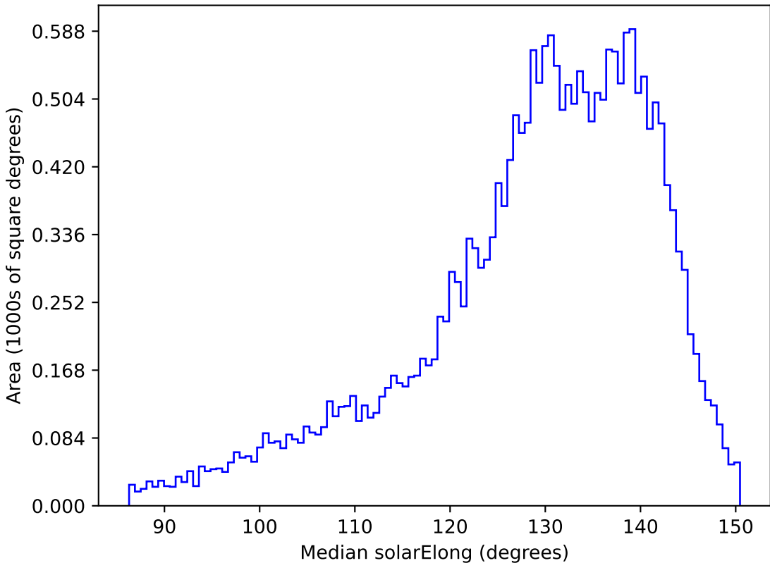
scp_reweight_v3.3_10yrs All sky y band: Median solarElong
