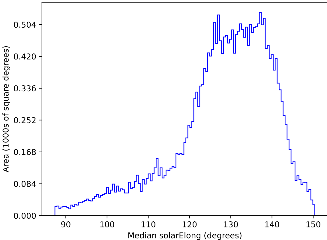
scp_reweight_v3.3_10yrs All sky i band: Median solarElong
